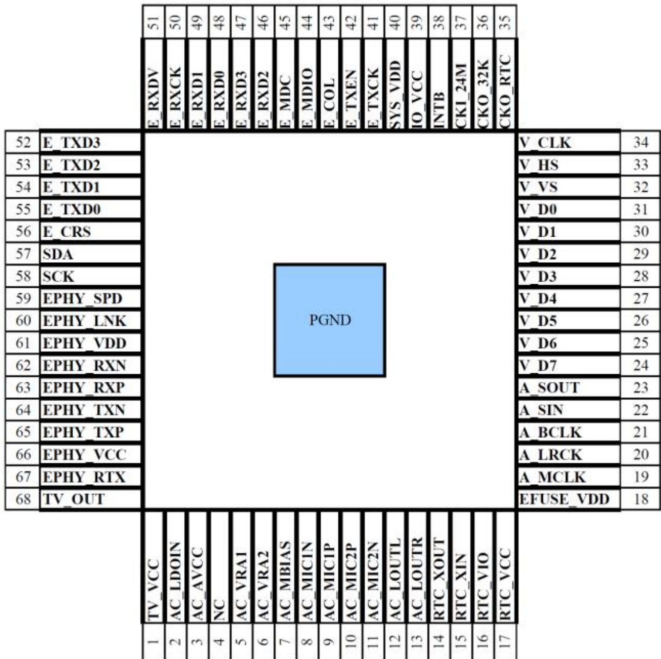
Figure 2. AC200 Pin Configuration
